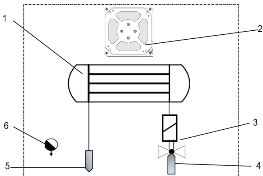
Figure 3 - Refrigerant circuit
