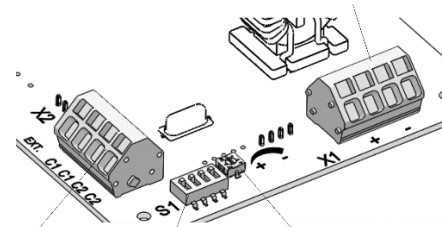
X2 External control input S1 Operating mode selection Light intensity control (15-100%)
