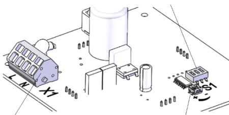
X1 Light intensity control Operating voltage connection (15 – 100%)
