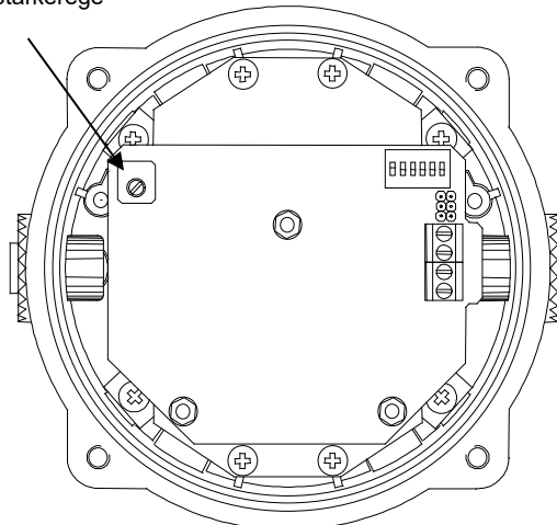
BExCS110-05D DC
