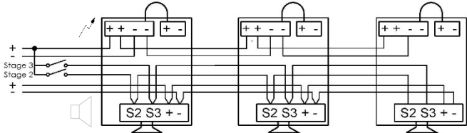
Fig 6b. BExCS110-05D DC Simplified Block Diagram for independent operation (positive switching)
