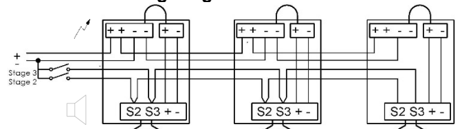
Fig 5a. BExCS110-05D DC Simplified Block Diagram for simultaneous operation (negative switching)
