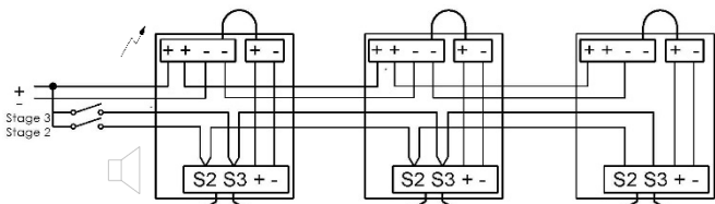
Fig 6a. BExCS110-05D DC Simplified Block Diagram for simultaneous operation (positive switching)
